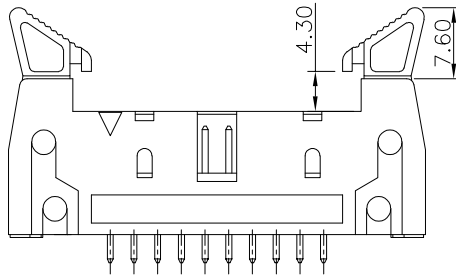
Short Ejector
