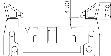
Short Ejector
