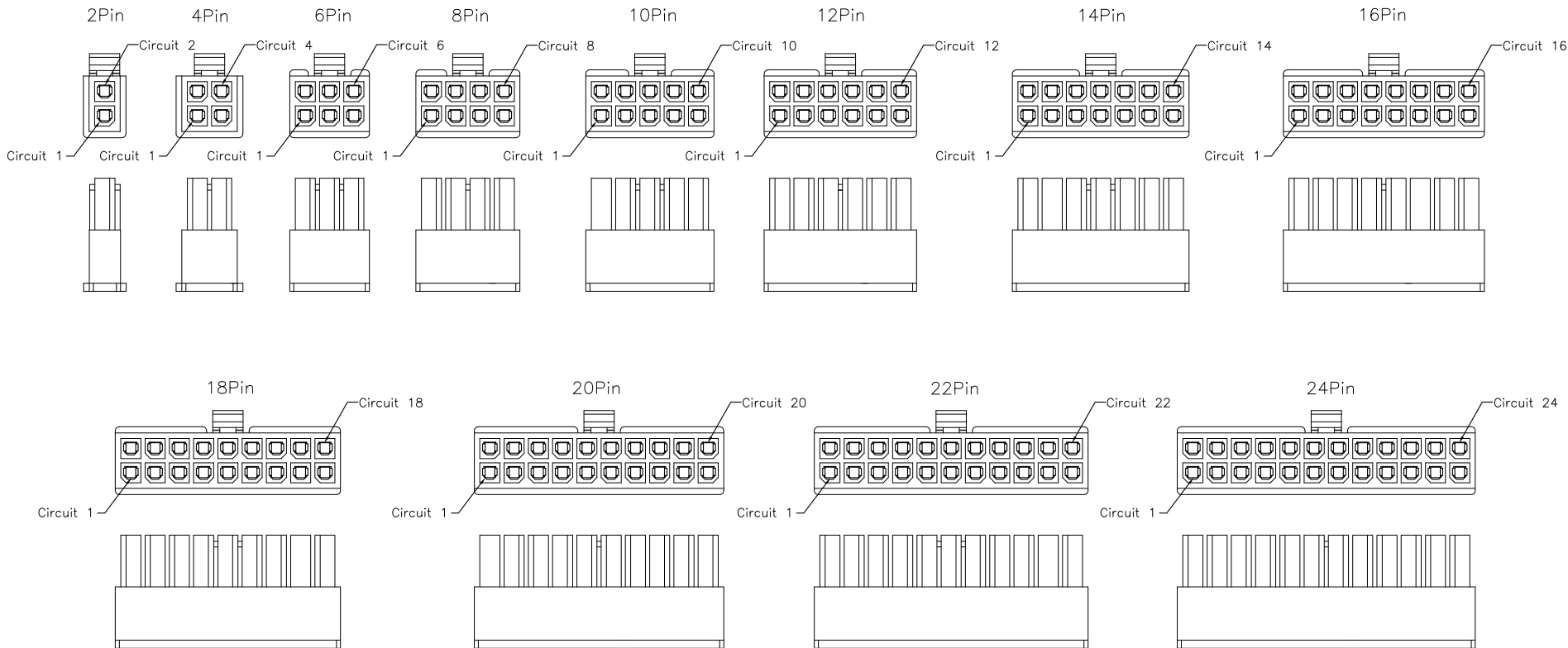
02~24P Protection Key Drawing(Ref.)
